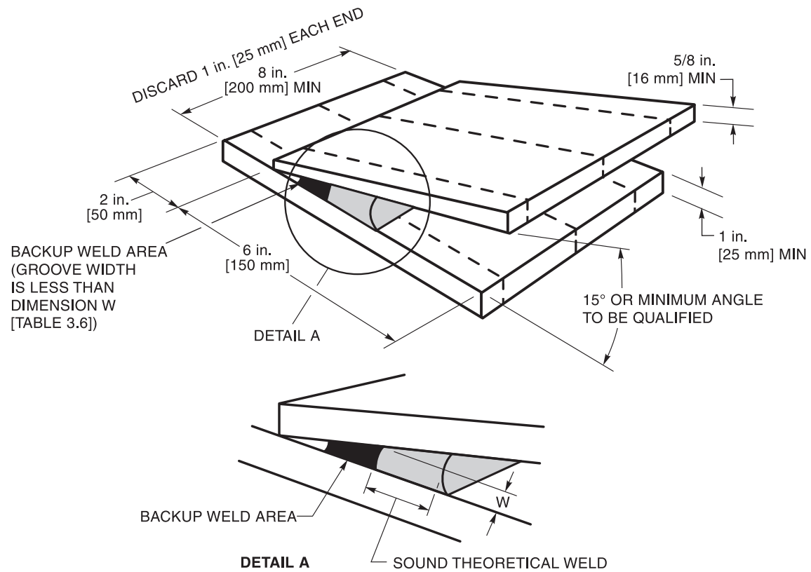
Figure 4.26—Acute Angle Heel Test (Restraints not Shown) (see 4.12.4.2)
