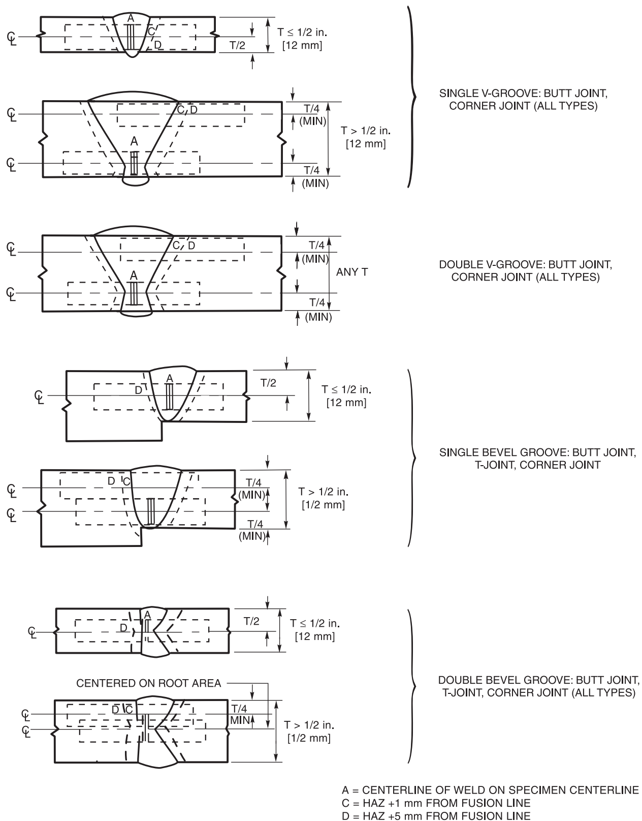
Figure III-1—CVN Test Specimen Locations (see III.2.1)
