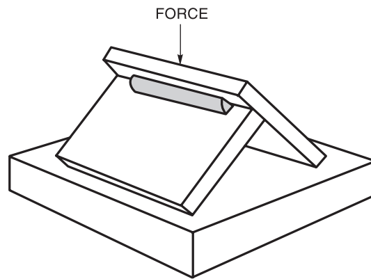
Figure 4.34—Method of Rupturing Specimen—Tack Welder Qualification (see 4.31)
