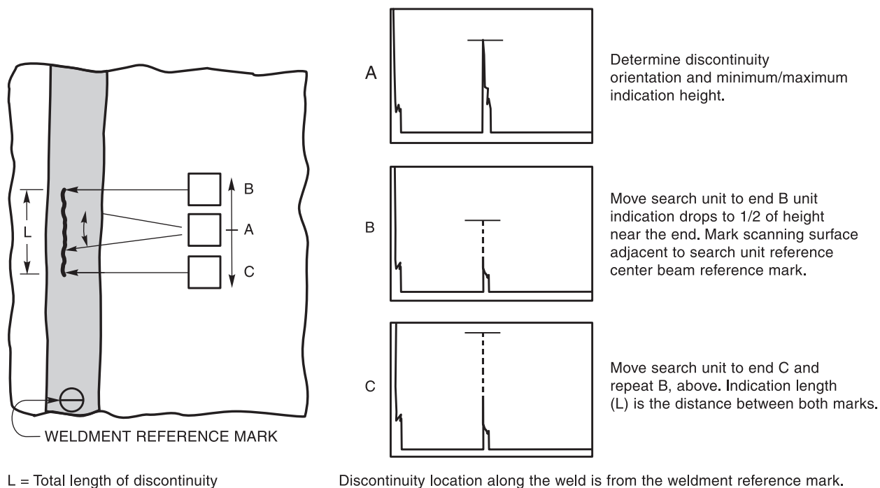
Figure K-13—Discontinuity Length Dimension (see K9.3)
