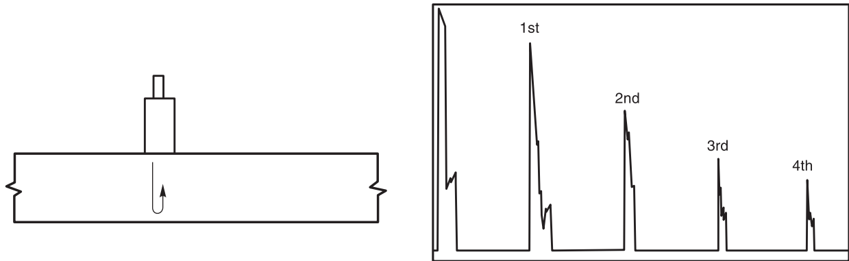
Figure K-5—Compression Wave Depth (Horizontal Sweep Calibration) (see K6.2.1)
