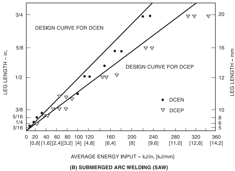
Figure XI-4—Relation Between Fillet Weld Size and Energy Input (see XI6.1.5)
