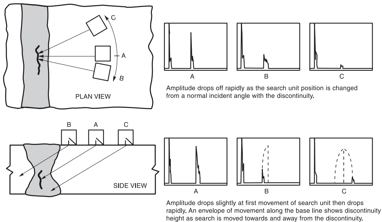
Figure K-11—Planar Discontinuity Characteristics (see K8.2.3)
