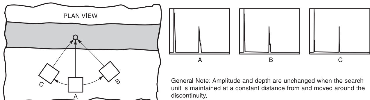
Figure K-9—Spherical Discontinuity Characteristics (see K8.2.1)
