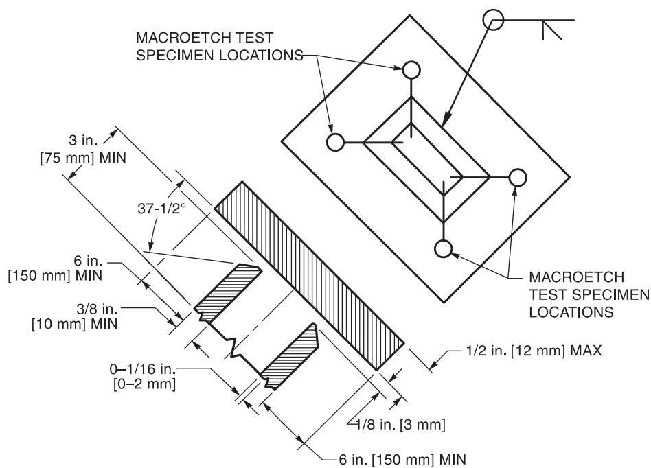
Figure 4.28—Corner Macroetch Test Joint for T-, Y-, and K-Connections without Backing on Box Tubing for CJP Groove Welds— Welder and WPS Qualification (see 4.12.4.1 and 4.26)
