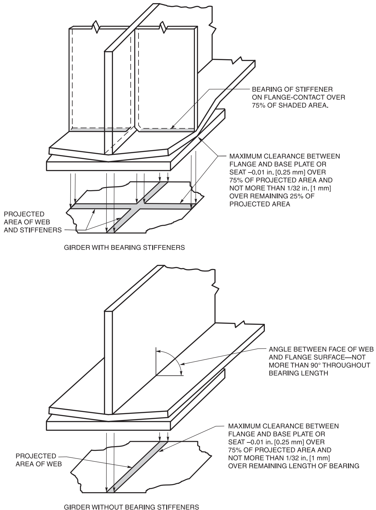
Figure C5.8—Tolerances Bearing Points (see C5.23.10)
