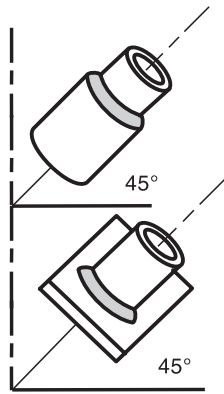
(A) FLAT WELDING TEST POSITION 1F (ROTATED)
