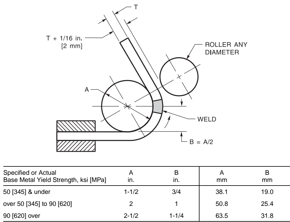
Figure 4.16—Alternative Wraparound Guided Bend Test Jig (see 4.8.3)
