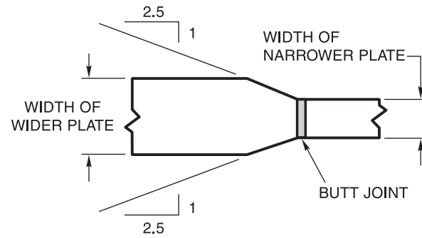
Figure 2.3—Transition of Widths (Statically Loaded Nontubular) (see 2.7.1 and 2.16.1.1)
