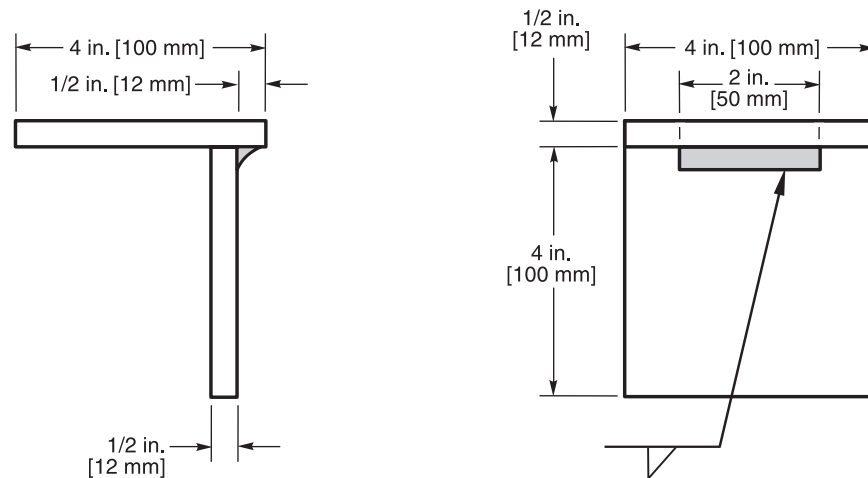
Figure 4.38—Fillet Weld Break Specimen—Tack Welder Qualification (see 4.19.2)
