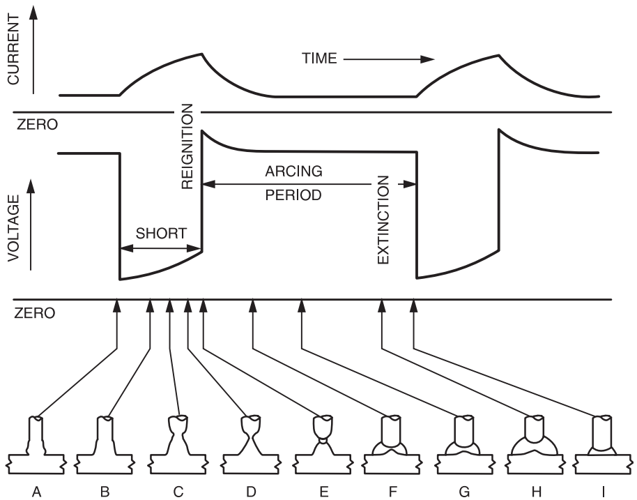
Figure A-1—Oscillograms and Sketches of GMAW-S Metal Transfer
