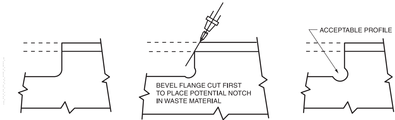
Figure C5.2—Examples of Good Practice for Cutting Copes (see C5.17)
