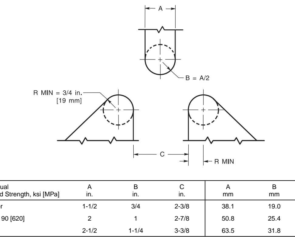
Figure 4.17—Alternative Roller-Equipped Guided Bend Test Jig for Bottom Ejection of Test Specimen (see 4.8.3)
