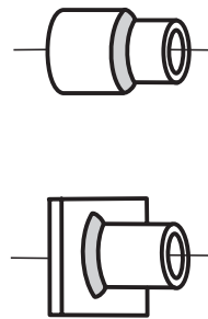
(E) MULTIPLE WELDING TEST POSITION 5F (FIXED)
