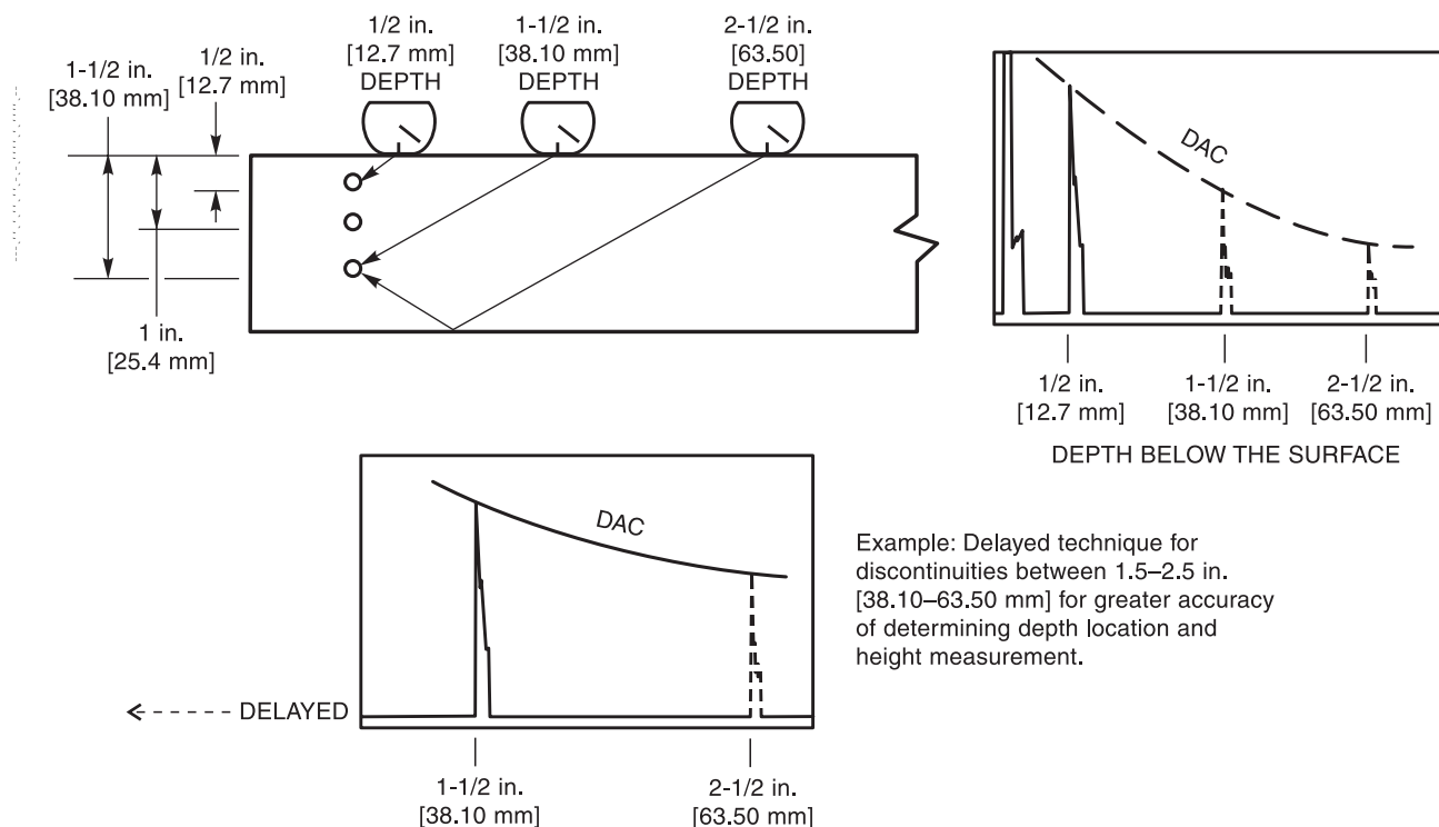
Figure K-7—Shear Wave Distance and Sensitivity Calibration (see K6.3.1)
